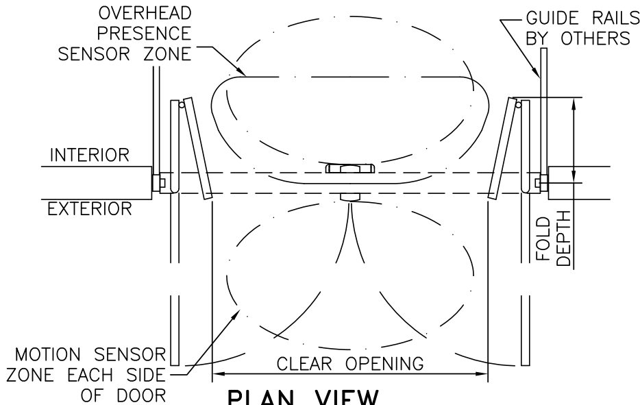
PLAN VIEW SCALE: 3/8" = 1'-0" FOLD-IN
