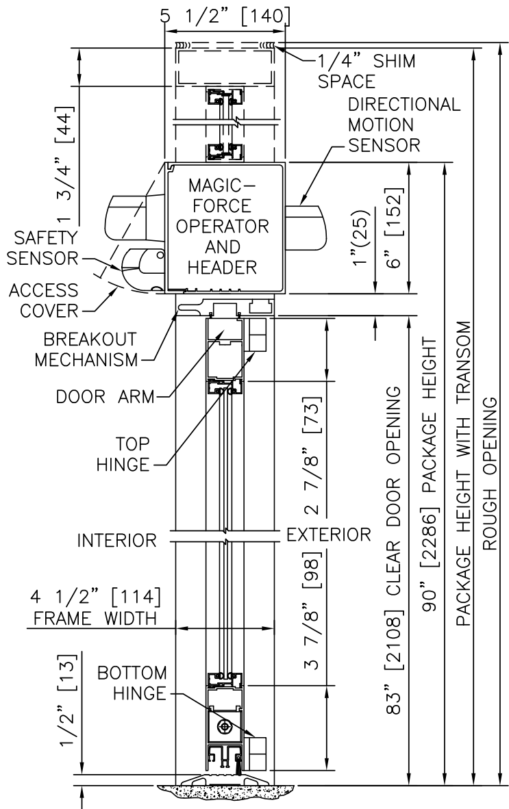
VERTICAL SECTION SCALE: 2" = 1'-0" FOLD-IN
