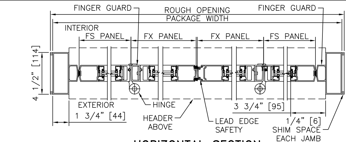
HORIZONTAL SECTION SCALE: 2" = 1'-0" FOLD-IN
