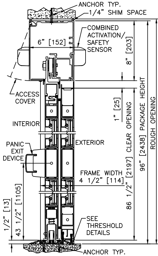
1 VERTICAL SECTION
