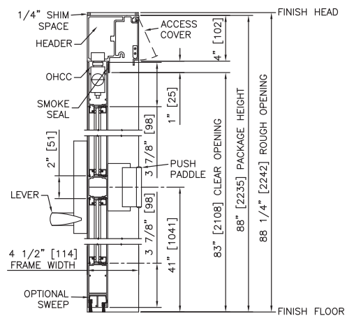
VERTICAL SECTION (4" HEAD)
