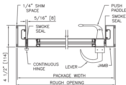
HORIZONTAL SECTION (SINGLE)
