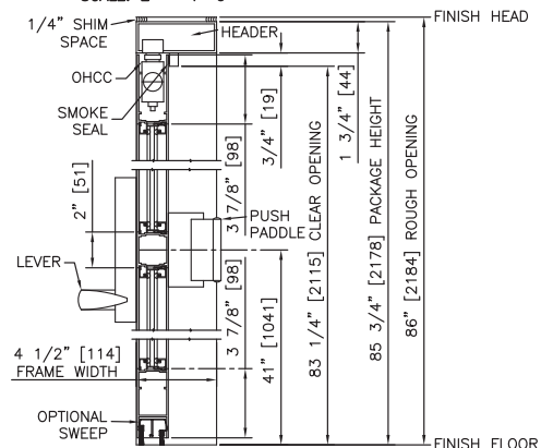
VERTICAL SECTION (1 3/4" HEAD)
