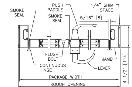
HORIZONTAL SECTION (UNEVEN PAIR)
