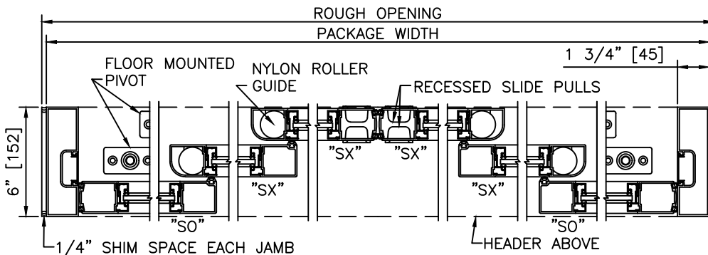
2 HORIZONTAL SECTION
