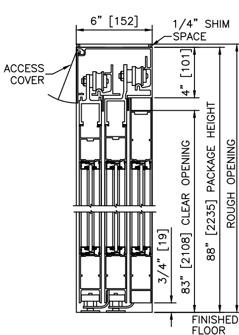
1 VERTICAL SECTION
