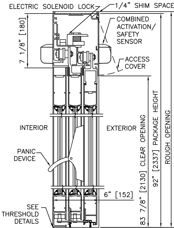
1 VERTICAL SECTION
